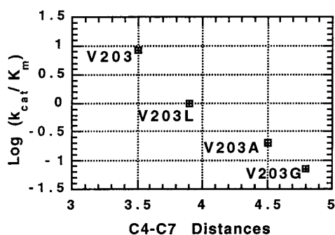
FIGURE 5: Catalytic efficiency ( k_{cat}/K_m ) of HLADH as a function of close contact distance between C4 of NAD^+ and C7 of PhCH_2OH for wild-type Val203 and single point mutants. Values of k_{cat}/K_m are from the literature (19, 21), and the distances are from MD simulations.
