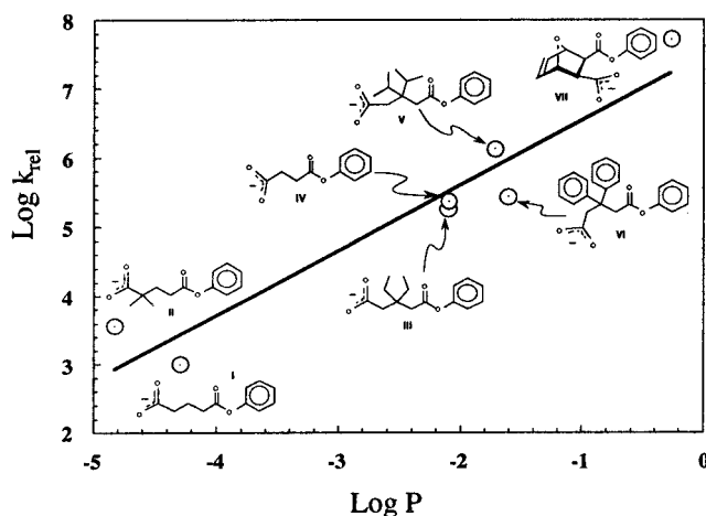
FIGURE 2: Log of the relative rate constants ( k_{\text{rel}} ) for anhydride formation from mono- p -bromophenyl esters vs the log of the probability ( P ) for NAC formation of each monophenyl ester of the various dicarboxylic acids.
